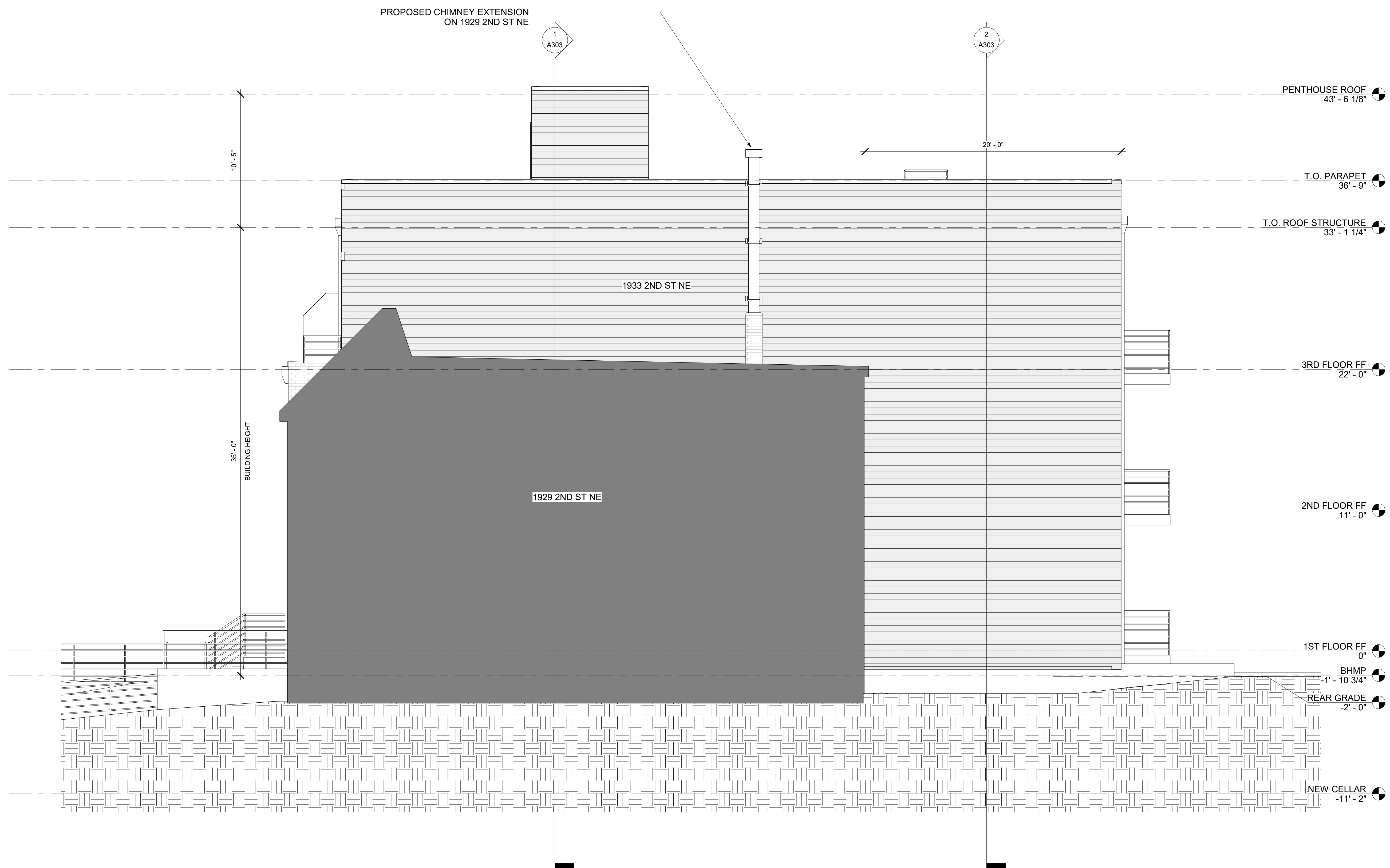
1 SOUTH ELEVATION A100/A202 1/4" = 1'-0"
